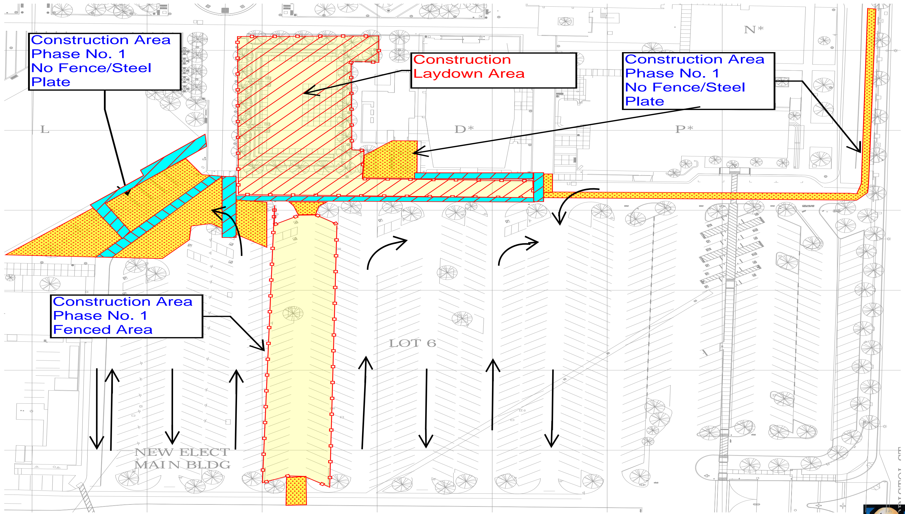
CONSTRUCTION PHASE NO 1 - LOGISTICS MAP (PRELIMINARY 11.16.15) Santa Ana College - Parking Lot 6 November 23, 2015 to March 3, 2016 (Subject to change)
